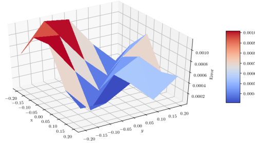
Figure 6: Error on the two dimensional case.
